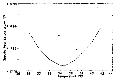
Fig. 1 Specific heat of water as a function of temperature.
