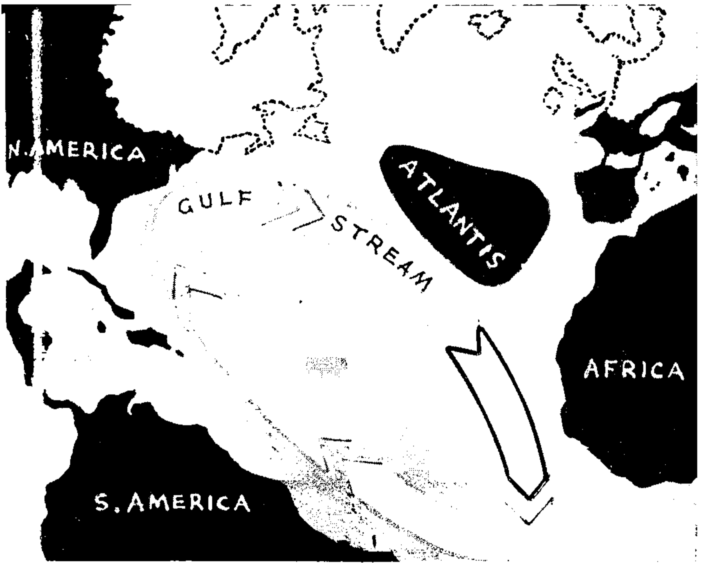
ABOVE: Blocking the Gulf Stream, Atlantis might have been the cause of the last Ice Age in Europe and America. BELOW: The sinking of Atlantis 12,000 years ago (according to Plato) could have ended the Ice Age by letting the warm Gulf Stream advance northward to become "central heating" for Europe.
